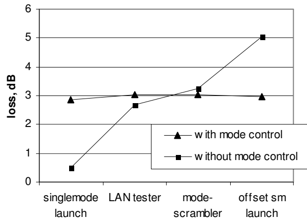
Fig. 7 Insertion loss of eleven concatenated patchcords
