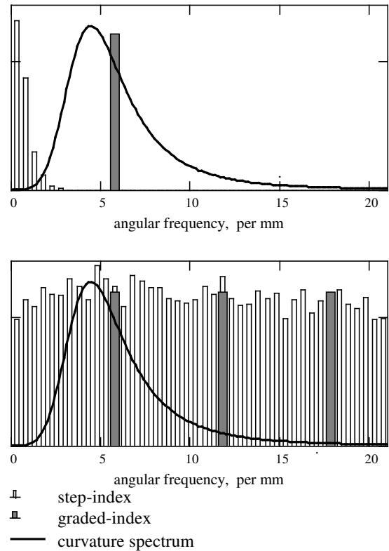
Fig. 1 Curvature spectrum of point-load mode-scrambler, and \Delta\beta spectrum for coupling between modes in step and graded-index fibres: (a) adjacent modes, (b) all modes.
