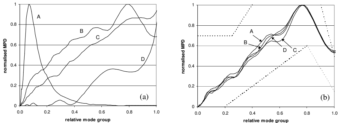
Fig. 8 Measured MPDs, (a) direct from source, (b) after mode controller. A: singlemode launch, B: LAN tester, C: mode-scrambler, D: offset singlemode launch.
