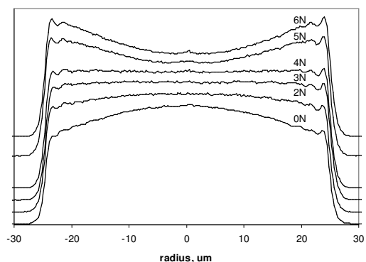
Fig. 2 Near-field profiles of 50um step-index fibre vs point loading.
