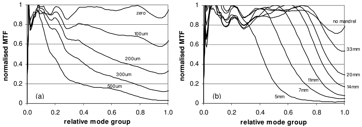
Fig. 4 MTFs of (a) longitudinal filter, vs air gap, and (b) mandrel-wrap filter, vs mandrel diameter.
