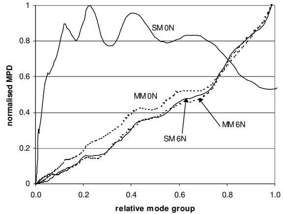
Fig. 3 Measured MPDs of graded-index fibre spliced to point-load mode-scrambler, for singlemode (solid) and multimode (dotted) launches.
