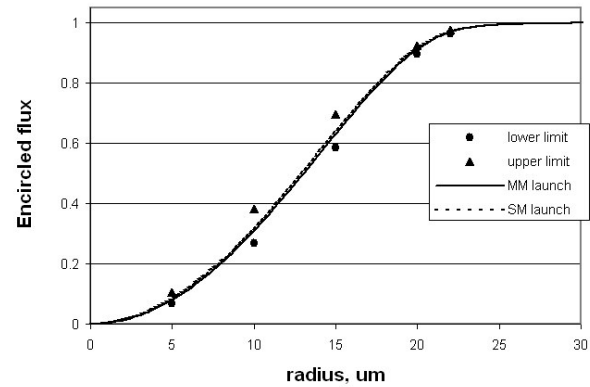
Fig. 9 Encircled flux template, draft IEC61280-4-1.
