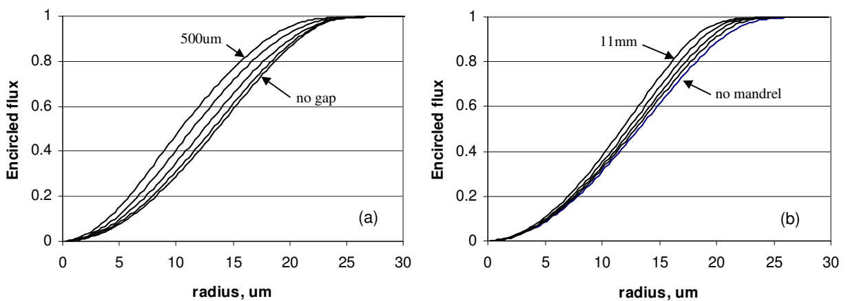
Fig. 5 Encircled flux of (a) longitudinal filter, vs air gaps of zero, 100μm, 200μm, 300μm 500μm, and (b) mandrel-wrap filter, vs mandrel diameters of no mandrel, 33mm, 20mm, 14mm, 11mm.
